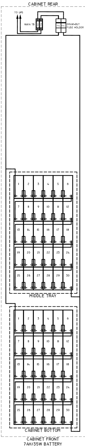
BCI4 TYPICAL WIRING (PLEASE CONSULT FACTORY FOR ADDITIONAL CONFIGURATIONS)
