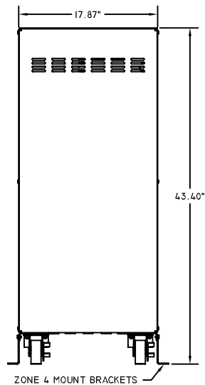
ZONE 4 MOUNT BRACKETS FRONT VIEW
