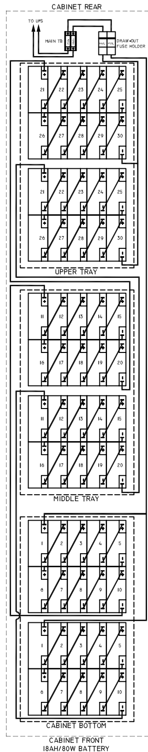
BCI4 TYPICAL WIRING (PLEASE CONSULT FACTORY FOR ADDITIONAL CONFIGURATIONS)
